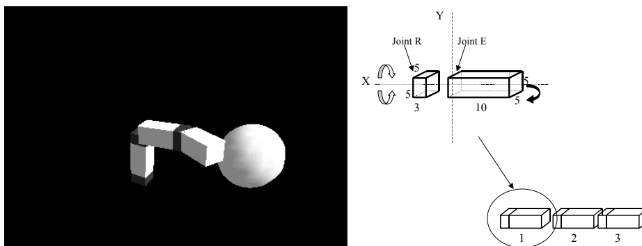
Figure 1. Left: The artificial finger and a spherical object. Right: A schematic representation of the finger.
