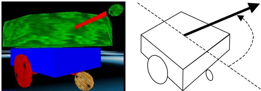
Figure 4. Left: A single s-bot. The upper and the lower part of the body represent the turret and the chassis, respectively. The larger and the smaller wheel represent the motorized and passive wheels, respectively. The line represents the link through which an s-bot is attached to another s-bot. Right: The traction force detected by the sensors of the s-bot. The dashed line indicates the frontal direction of the s-bot. The full arrow indicates the traction that the turret exerts on the chassis. The dashed arrow indicates the angle between the traction force and the frontal direction of the chassis.
